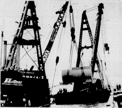
AT PORT NEWARK the "Century," the largest of three derrick barges recently acquired by the Hoffman Companies of Belleville, hoists a 440 ton stator of an electrical generator onto the "Monarch," second barge in the fleet.
